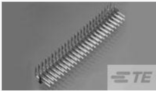
TE Part # 1-5176837-4 30 AMPMODU 2MM, H, AU, LF
