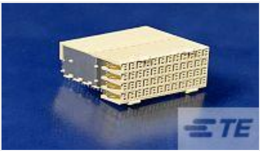
TE Part #6469286-1 HM-ZD 4PR RECP 96P
