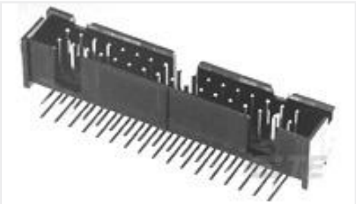
TE Part #1-5103311-2 A/L LOW PRO HDR 60P RA BLACK
