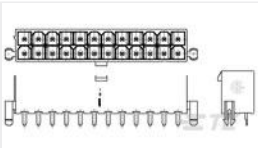
TE Part #5-103904-7 08 MTE HDR SRRA LATCH W/HLDWN
