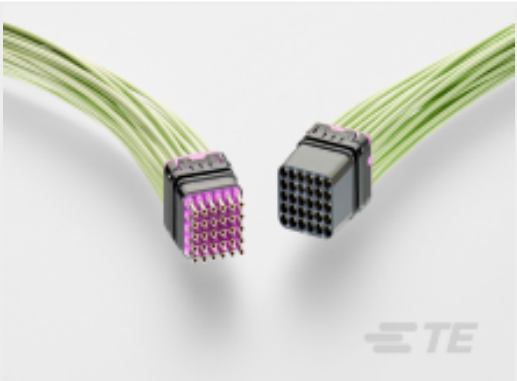
TE Part #ZPF000000000202888 DMC-MR 30-23 BA
