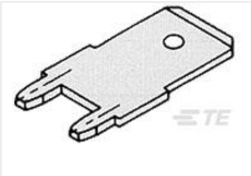
TE Part #1217566-1 250 FASTON,PCB TAB,TCBR
