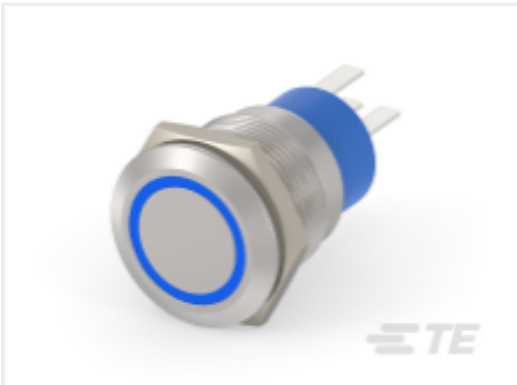
TE Part #1-2213764-9 AV19 SPM 3A FIX RING LED BLUE 24V
