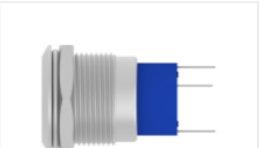
TE Part #2317404-1 AV19 SPM 3A FIXED RING R&G 12V
