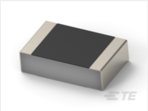
TE Part #9-2176453-9 CPF 0201 60K4 0.1% 25ppm 1K RL
