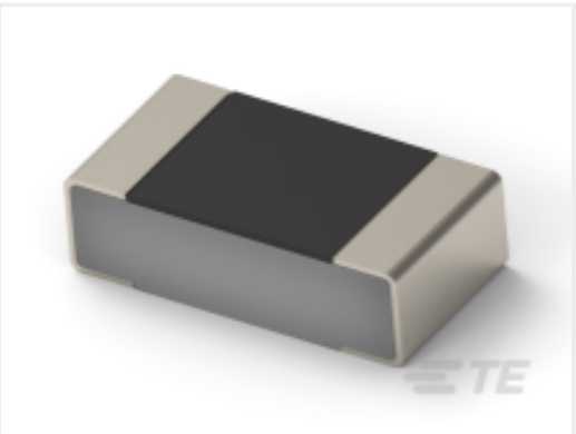
TE Part #2176467-6 TLRP 1206 1.0W R025 1% 50PPM 5K RL
