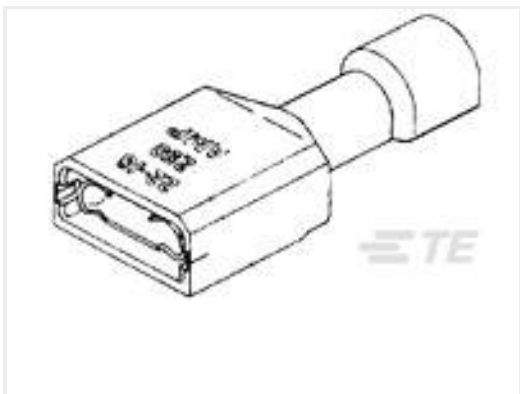
TE Part #3-350819-2 ULTRA-FAST 250 ASY REC 16-14 AWG TPBR
