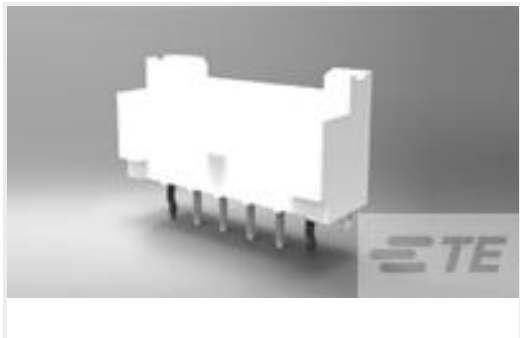
TE Part #1744418-3 3 POS EP 2.5 HDR, GLOW WIRE
