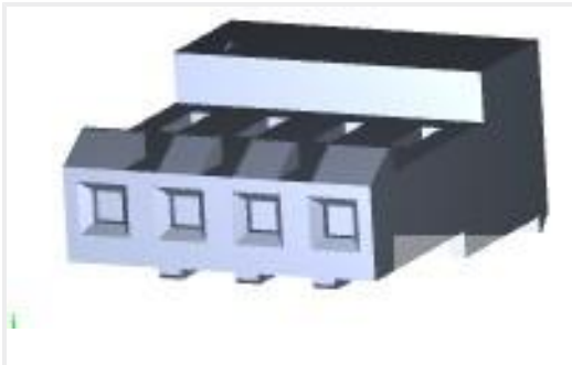
TE Part #3-641217-4 04P MTA156 CONN ASSY 18AWG ORA
