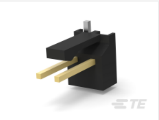
TE Part # 3-647167-2 02P MTA100 HDR ASSY SM 15AU LF
