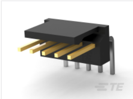
TE Part # 3-647079-5 05P MTA100 HDR FLRAFB 15AU LF
