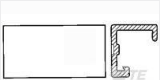
TE Part #1-640250-2 12P SL156 HSG W/LCK RAMP NATL
