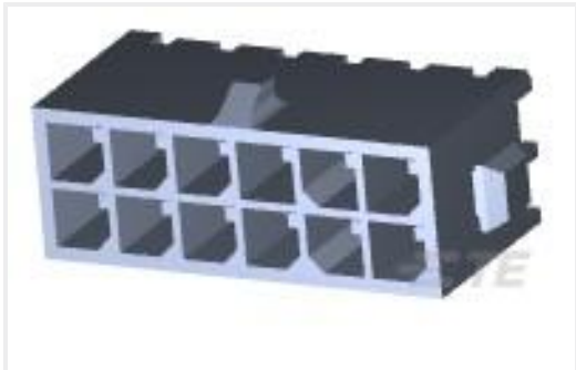
TE Part #4-794630-2 12P MICRO MNL ASSY,VRT,HDR,LF
