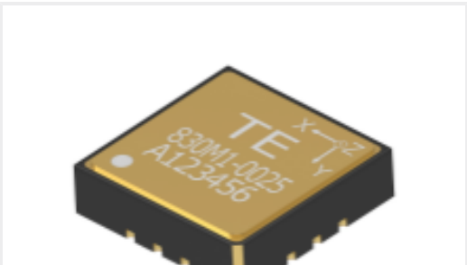
TE Part #CAT-EAC0023 Model 830M1 Triaxial SMT Accelerometers
