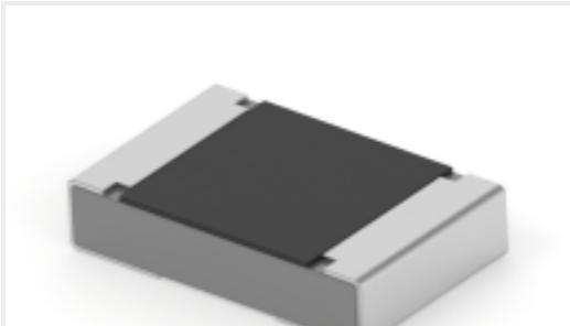
TE Part #5-2176478-8 RA73F 2A 23K2 0.1% 1K RL
