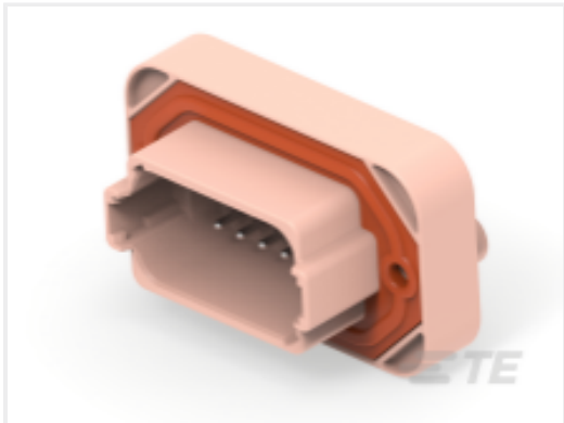
TE Part #DT15-12PD HDR, 12P, BRN, ST, NI/CU, D
