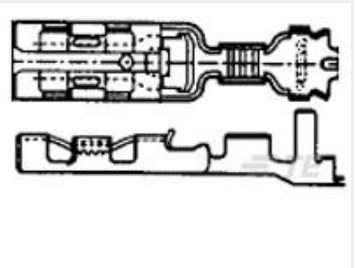
TE Part #353249-2 110 PL EX REC. 26-22AWG PTPHBZ
