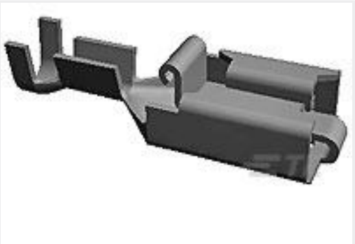
TE Part #341001-3 PL 250 REC TERMINAL 13-11 TPBR LP
