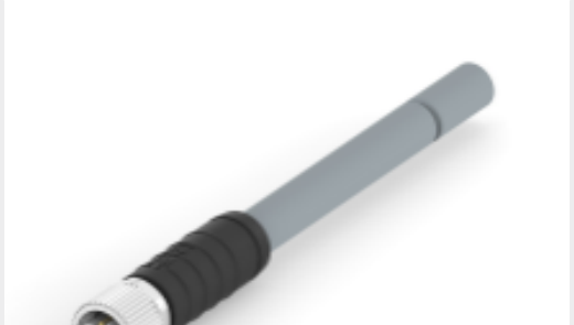
TE Part #T41513C9L25-002 RPC-M12L-5FS-1.0-PUR 16AWG GY
