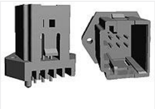
TE Part #953363-1 6pos MQS .63 header 180deg
