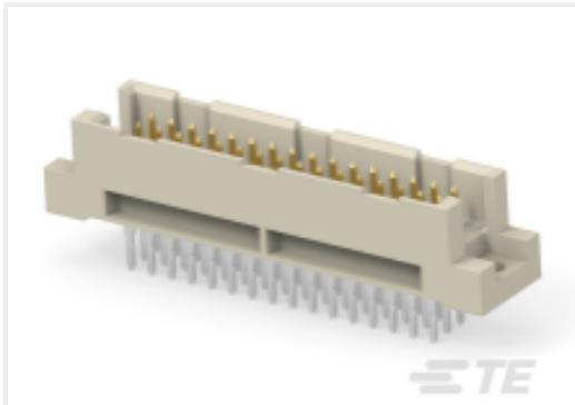
TE Part #354382-E STVR/2 48 MI ABC VV 4-00 EE 6,0 * 247 E
