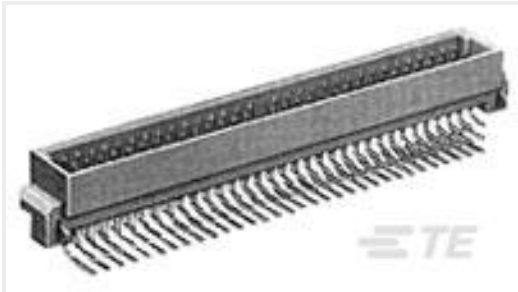
TE Part #5536416-5 ASSY,PIN,EURO,"C",LEAD-FREE,96
