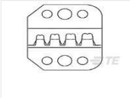
TE Part #58583-2 PROCIMP DIE SUPERSEAL 1.5 SER
