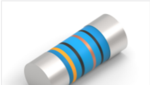
TE Part #7-2176315-5 MELF SMA-A 10R 1% 50PPM 0204 0.4 W
