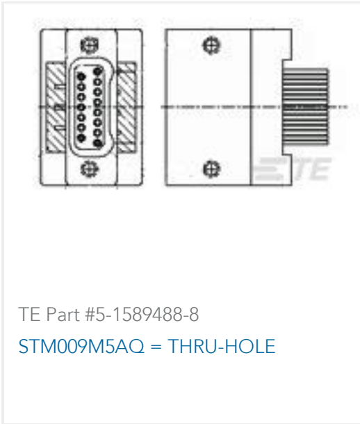
TE Part #CAT-STM-65SC DUALOBE Receptacle Connectors: Metal Shell, 65 Pin/2 row
