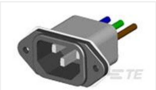
TE Part #1-6609987-1 15SRB8-R=F8220A
