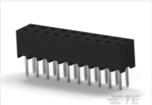
TE Part #2-2314820-0 20P,2MM,B-B,REC,DRV,T,2.7,0.1AU,TB
