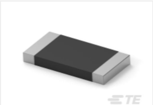
TE Part #7-2176422-5 TLRP 2512 3.0W R091 1% 50PPM 4K RL
