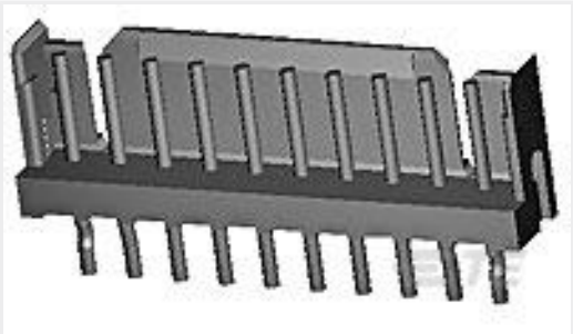
TE Part # 4-292161-2 CT P/HDR ASSY V 2P W/KINK YELL
