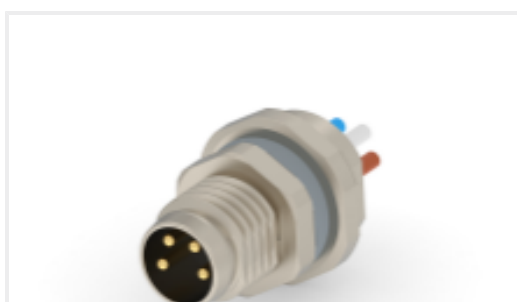
TE Part #T4070014041-001 M8, MLE, PNL REAR, 4 POS, STR WIRE
