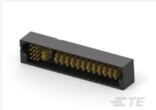
TE Part #6450821-6 MBXL VERT HDR 12S+2HDP+12LP
