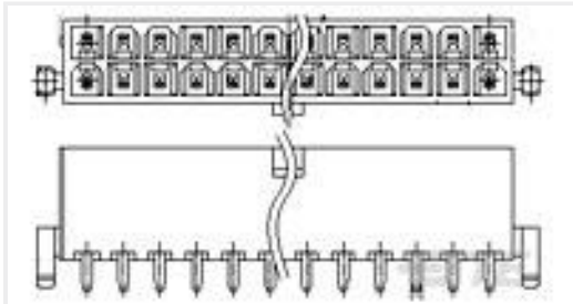
TE Part #2291931-2 CDFP RCPT CONNECTOR & CAGE STYLE 1
