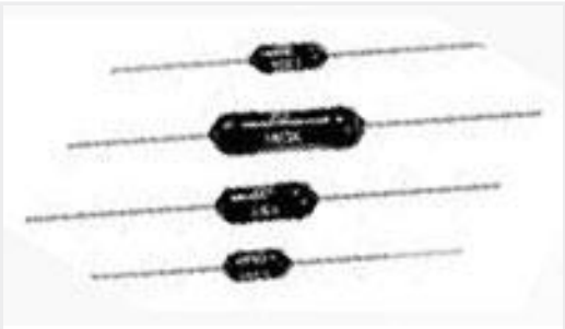
TE Part #4-1879665-3 H8 34K 0.1% 15PPM
