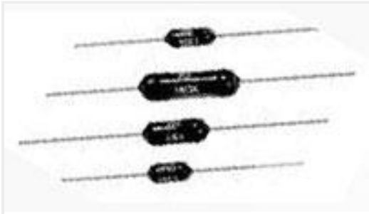
TE Part #1-1879663-5 H8 150R 0.1% 15PPM
