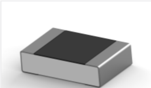
TE Part #8-2176380-9 RQ 0805 9K53 0.1% 10PPM 5K RL
