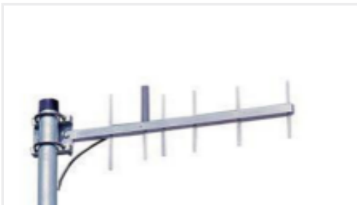
TE Part #PC906N Yagi, FWA, 12in, NF 896-940MHz, 8.5dBd
