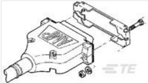
TE Part #5745583-1 UNIV SLIDLTCH KIT SZ 2
