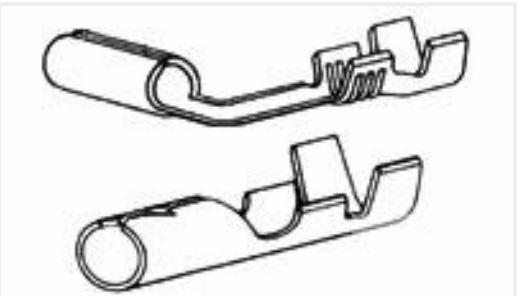
TE Part #42142-2 SHUR PLUG TERMINAL 18-14 AWG BR
