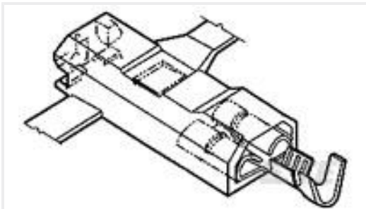
TE Part #521998-2 ULTRA-POD 250 ASSY REC 18-14 AWG TPBR
