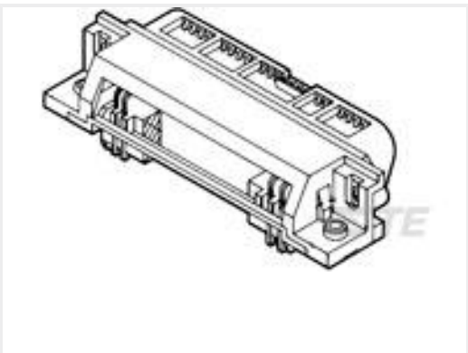
TE Part #5552791-1 ASSY,RCPT,24 POSN, RTANG PCB
