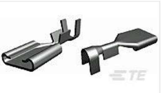
TE Part #42743-1 250 FASTON REC 22-18 AWG BR
