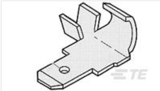
TE Part #42770-2 250 FASTON FLAG TAB 18-14 AWG TPBR
