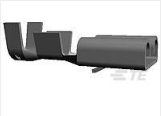
TE Part #60249-2 FF 250 REC 16-12AWG TPBR
