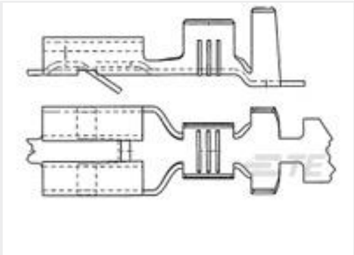
TE Part #281197-2 FF 187 REC 1.0-2.5MM2 PTBR
