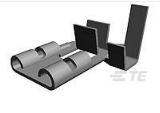
TE Part #63538-1 250 FASTON FLAG REC 18-14 BR
