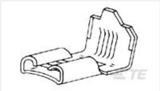
TE Part #62056-7 250 FASTON FLAG REC 18-12 AWG TPBZ
