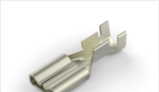
TE Part #2238199-3 FASTON 187 STD REC STR 18-14TPBR
