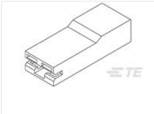
TE Part #521120-1 PL 250 HOUSING RECEPTACLE NYLON 6/6
