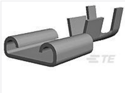
TE Part #2-160256-1 250 FASTON,REC.,17-14 AWG,BR
