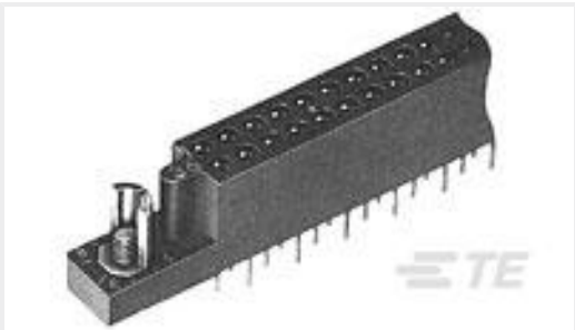
TE Part #530340-7 2 ROW BOX RECP 90 POS STAG
