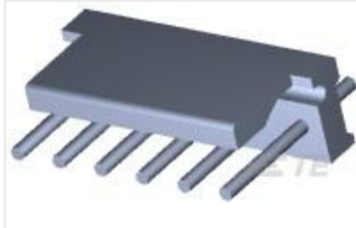
TE Part #3-641209-6 06P MTA156 HDR ASSY FL ST LF
