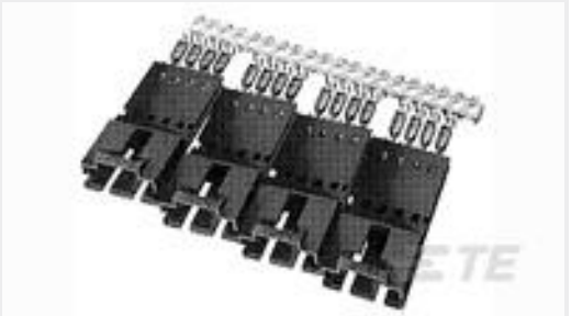
TE Part #5-103945-3 4X4 MTE SHRD PIN SR LATCH .100
