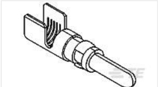
TE Part #213845-4 PWRBAND PIN ASY 14-12 L.P.
