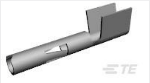
TE Part #640310-3 UMNL SOK 12-10 PTPPHBZ
