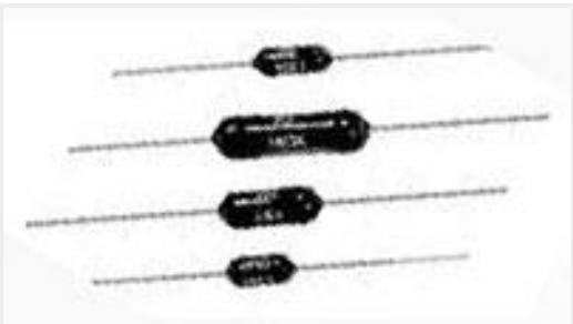
TE Part #1-1879665-6 H8 17K8 0.1% 15PPM
