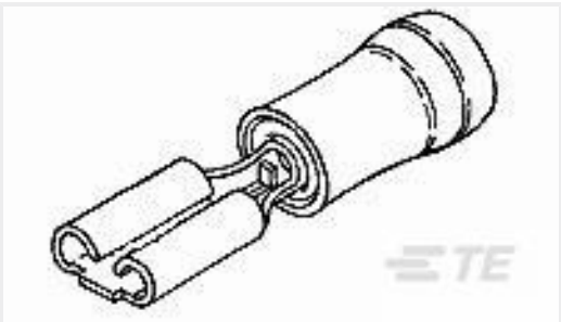
TE Part #8-61060-1 RECEPT,IDG FASTON 22-18 110
